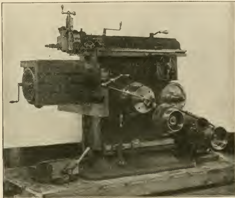
POTTER & JOHNSTON'S MOTOR-DRIVEN SHAPER.
